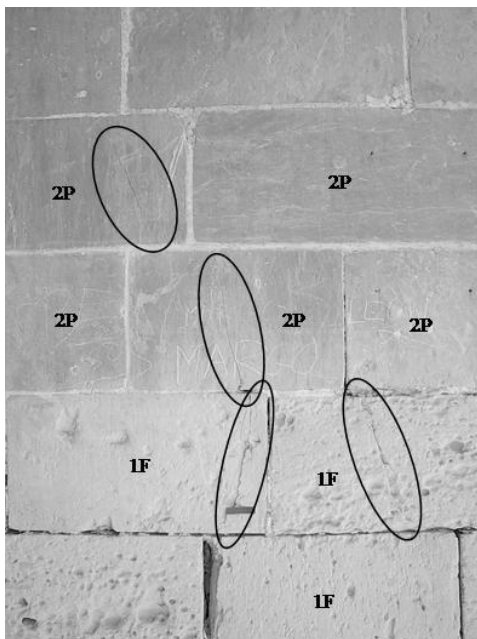
Figure 10. Auberge de Castille, Valletta, south corner: tensile fractures (circled) related to loss or differential deformation of mortar. Stone types labelled, also showing different forms of salt weathering.
